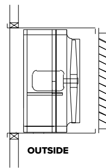
BOX MOUNTED THROUGH WALL/SHUTTER MOUNTED TO OUTSIDE OF BOX
