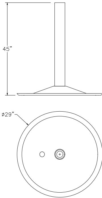
Pedestal Base
