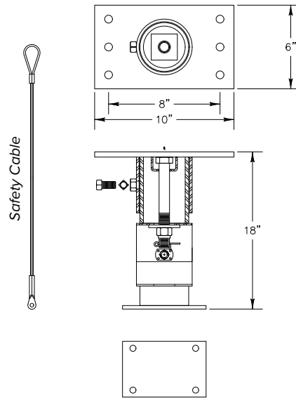
Vertical Mounting Bracket (Non-Oscillating)
